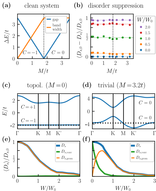
FIG. 2. Disorder-induced suppression of the superfluid weight in the extended Kane-Mele model [40]. (a) Evolution of the energy gap and the bandwidth of the lower band as a function of M . C is the Chern number of the lower spin-up band. (b) D_s as a function of M for different values of W/W_0 and \nu = 1/2 . The vertical dotted black line indicates the topological transition in the clean system. (c), (d) Energy bands of the clean systems along high-symmetry lines of the Brillouin zone for M values corresponding to topologically distinct cases. The dotted black lines indicate the Fermi level corresponding to \nu = 1/2 . (e), (f) \langle D_s \rangle as a function of W/W_0 for \nu = 1/2 .
