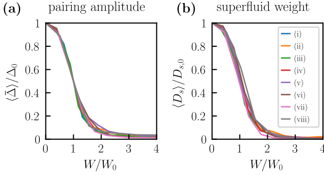
FIG. 1. Universality of the disorder-induced suppression of the pairing amplitude and the superfluid weight across a variety of lattice models [40]: (i)-(v) topological and trivial extended Kane-Mele models, (vi)-(viii) trivial single-band models (see text and SM [41] for details). The ensemble averages of (a) the spatial average of the pairing amplitude \bar{\Delta} and (b) the superfluid weight D_s are shown as a function of the disorder strength W/W_0 .
