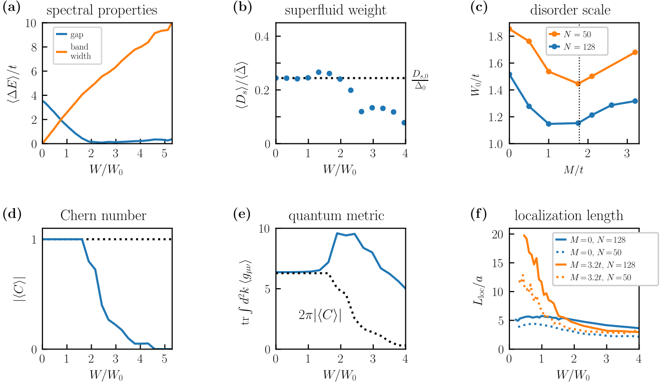
FIG. S2. Disordered Kane-Mele model with optimized flatness: (a) Evolution of the band gap and the bandwidth of the lower band as a function of disorder W . (b) Relation between full superfluid weight D_s and sample-averaged superconducting order parameter \bar{\Delta} . (c) Disorder scale W_0 as a function of the staggered on-site potential M for two different system sizes N . The dotted black line indicates the topological transition in the clean system. (d) Evolution of the Chern number of the lower spin-up band. (e) Evolution of the trace of the quantum metric of the lower spin-up band integrated over the Brillouin zone. The dotted black line indicates the evolution of the lower bound on this integral given by the Chern number C . (f) Localization length as a function of the disorder parameter W for the flat ( M = 0 ) and for a trivial ( M = 3.2t ) Kane-Mele model for two different system sizes N . The localization length is given in units of the sublattice separation a of the honeycomb lattice.
