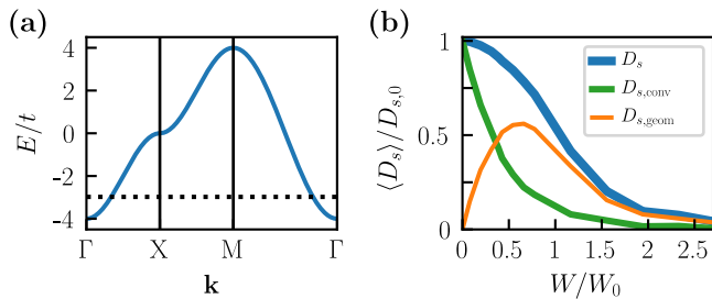
FIG. 3. Disorder-induced suppression of \langle D_s \rangle in a single-band model [40]. (a) Energy band dispersion of the clean system along high-symmetry lines of the Brillouin zone. The dotted line indicates the Fermi level at \nu = 1/5 . (b) \langle D_s \rangle , \langle D_{s,\text{conv}} \rangle and \langle D_{s,\text{geom}} \rangle as a function of W at \nu = 1/5 .
