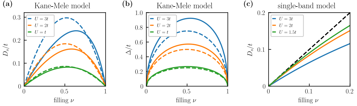
FIG. S8. Comparison with analytical formulas for the clean systems in the zero-temperature limit: (a) superfluid weight D_s and (b) superconducting order parameter \Delta of the flat Kane-Mele model for different coupling constants U as a function of the filling \nu . Solid lines represent the respective quantities as obtained directly from numerics, dashed lines show the results computed using Eqs. (S57) and (S58), respectively. (c) Superfluid weight of the single-band model for different U at small fillings close to the band bottom. Solid lines are the numerical results while the dashed black line represents the analytical result using Eq. (S56) assuming a parabolic band.
