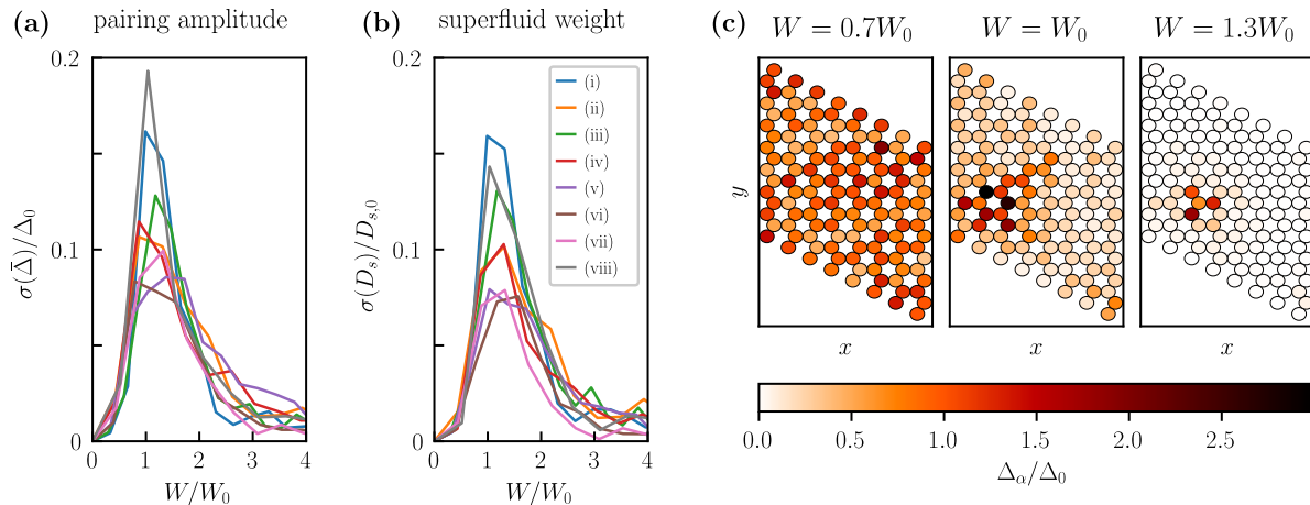
FIG. S5. Ensemble standard deviations \sigma of (a) the pairing amplitude \bar{\Delta} (spatial average) and (b) the superfluid weight D_s as a function of W/W_0 for the models considered in Fig. 1 of the main text: (i)-(v) topological and trivial extended Kane-Mele models, (vi)-(viii) trivial single-band models. (c) Spatial profile \Delta_\alpha of the pairing amplitude for single disorder realizations of the flat Kane-Mele model [model (i)] at different disorder strengths W/W_0 . White corresponds to a vanishing pairing amplitude, whereas darker colors signify a larger values. Around W = W_0 , the superconductor breaks up into isolated superconducting islands accompanied by large fluctuations of \bar{\Delta} and D_s .
