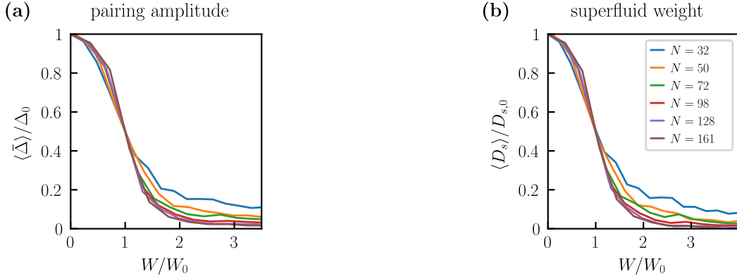
FIG. S6. Disorder-induced suppression of the pairing amplitude and the superfluid weight for different cluster sizes. We show results for the extended Kane-Mele model with flat lower band and U = 3t , T = T_{c,0}/100 , and \nu = 1/2 .
