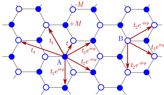
FIG. S1. Illustration of the extended Kane-Mele model on the honeycomb lattice with nearest-neighbor hopping t , i -th neighbor hopping amplitudes t_i , and staggered on-site potential M . Hopping processes between second neighbors acquire a phase e^{\pm i\sigma\varphi} depending on the spin \sigma = \pm 1 \equiv \uparrow, \downarrow of the involved particles, on the hopping direction, and on the sublattice A, B. Red arrows indicate a selection of hopping processes. Other hopping processes can be inferred by symmetry.
