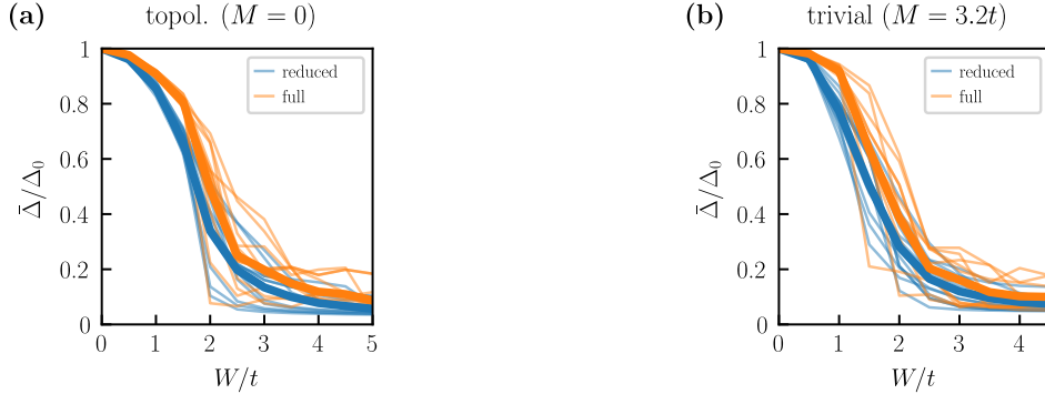
FIG. S7. Comparison between full (orange) and reduced (blue) mean-field approach for the superconducting order parameter \bar{\Delta} in the extended Kane-Mele model with U = 3t , T = T_{c,0}/100 , and \nu = 1/2 : (a) topological phase and (b) trivial phase. We show results of single disorder realizations (thin lines) and their ensemble averages (bold lines).
