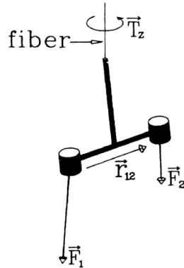
Figure 1. Operating principle of the Eötvös torsion balance. This idealized balance consists of two test bodies attached to a rigid, massless frame that is supported by a perfectly flexible torsion fibre. F_1 and F_2 denote the external forces on the test bodies. The torque about the fibre axis is T_z = (\mathbf{F}_1 \times \mathbf{F}_2 \cdot \mathbf{r}_{12})/|\mathbf{F}_1 + \mathbf{F}_2| . The signal is the change in T_z when the instrument is rotated about the fibre axis so that the component of \mathbf{r}_{12} along the direction of \mathbf{F}_1 \times \mathbf{F}_2 changes sign.
